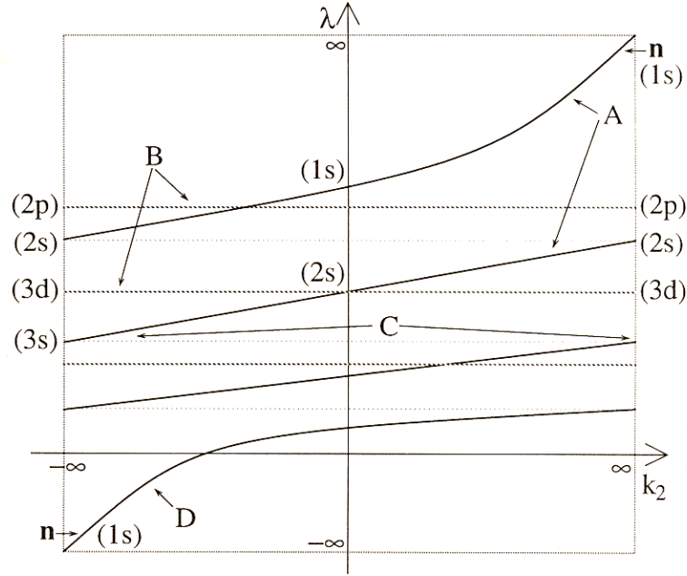
Figure 6. General spectrum of eigenvalues of \mathbf{Q} + k_2 \mathbf{J} as a function of k_2 . A: Eigenvectors with non-zero DC component (solid lines) vary with k_2 , and have eigenvalues that increase monotonically with k_2 . B: Eigenvectors with zero DC component (thick dotted lines) are independent of k_2 . C: Adjacent DC eigenvalues share a common asymptote (thin dotted lines). D: There is only one negative eigenvalue. The leading eigenvector at k_2 = \infty and the negative eigenvector at k_2 = -\infty are both equal to the DC vector, \hat{n} . The annotations in parentheses identify the eigenvectors of Linsker's system at layer \mathcal{B} \rightarrow \mathcal{C} . From [6].
